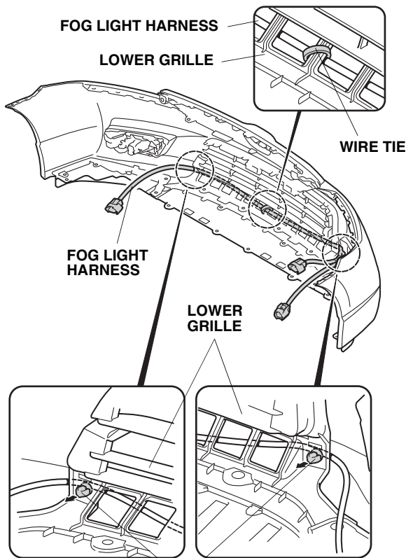
FOG LIGHT HARNESS CLIPS (Attach them to the hole on the lower grille.)
